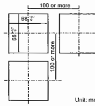
Panel cutout drawing
