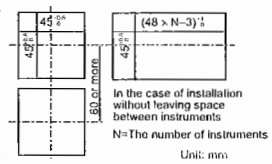
Panel cutout drawing
